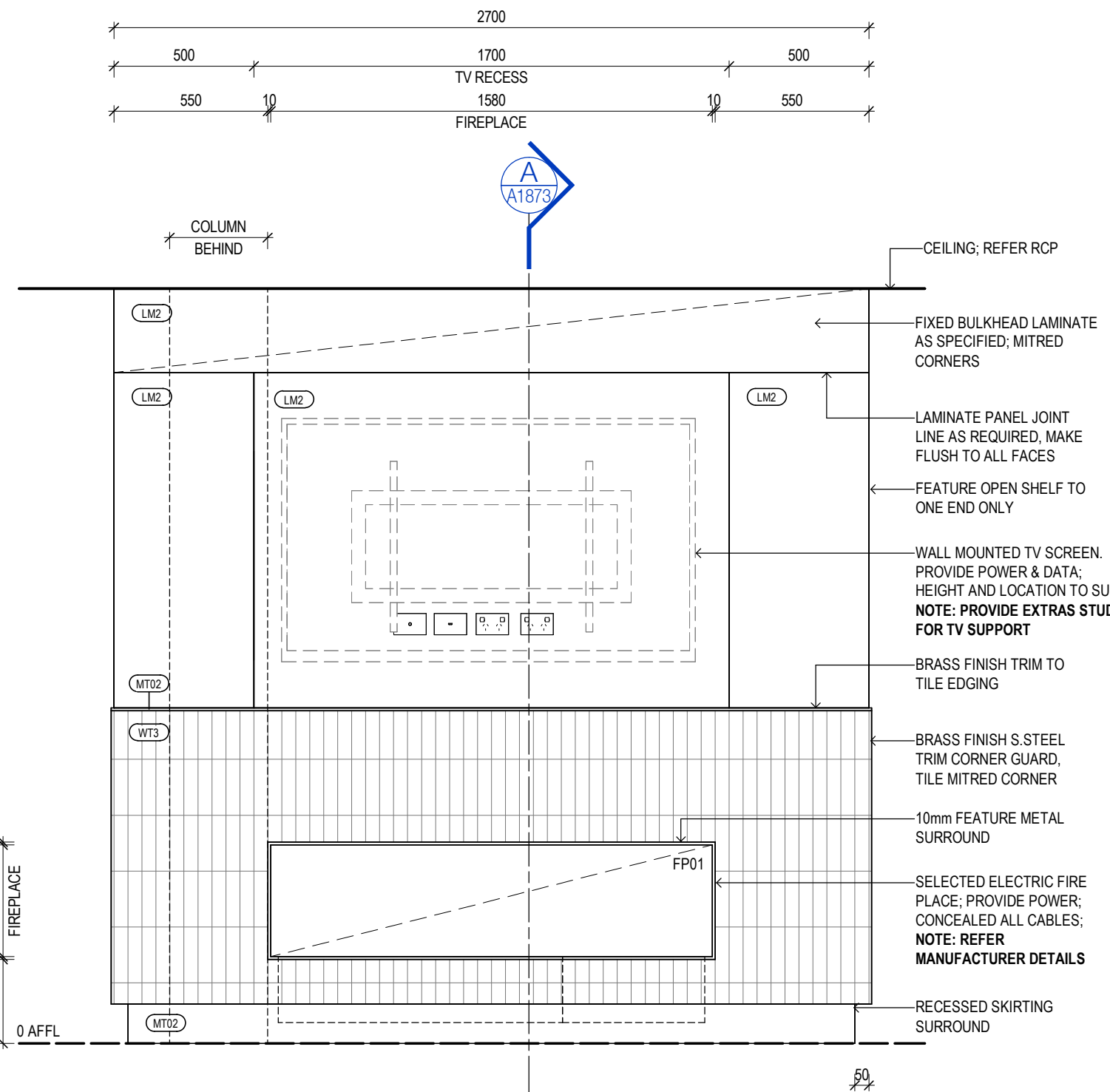
J-04 - Sports Bar Joinery - Lounge Side ELEVATION 4 Scale 1 : 20
