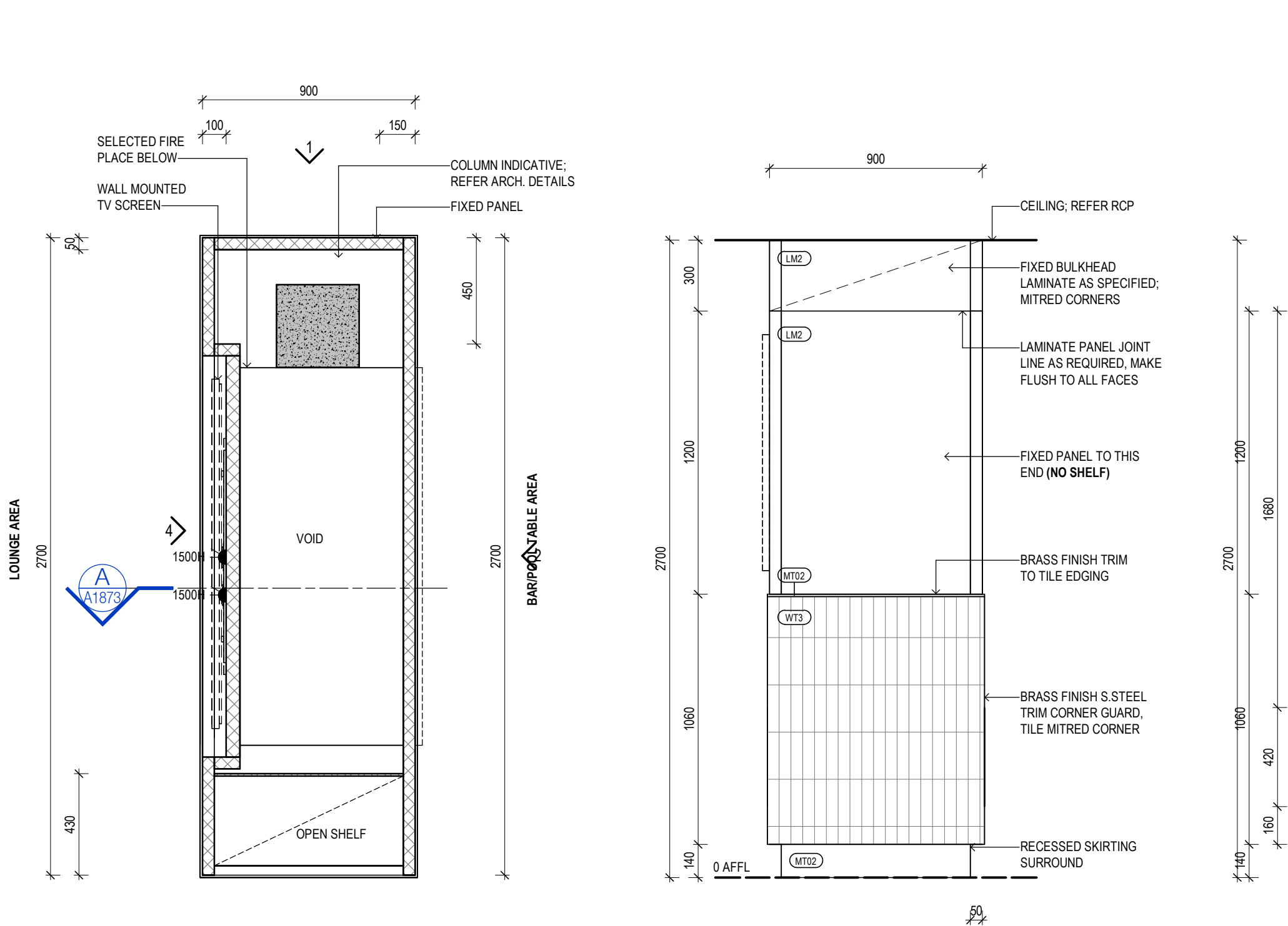
1 J-04 - SPORTS BAR JOINERY Scale 1 : 20
