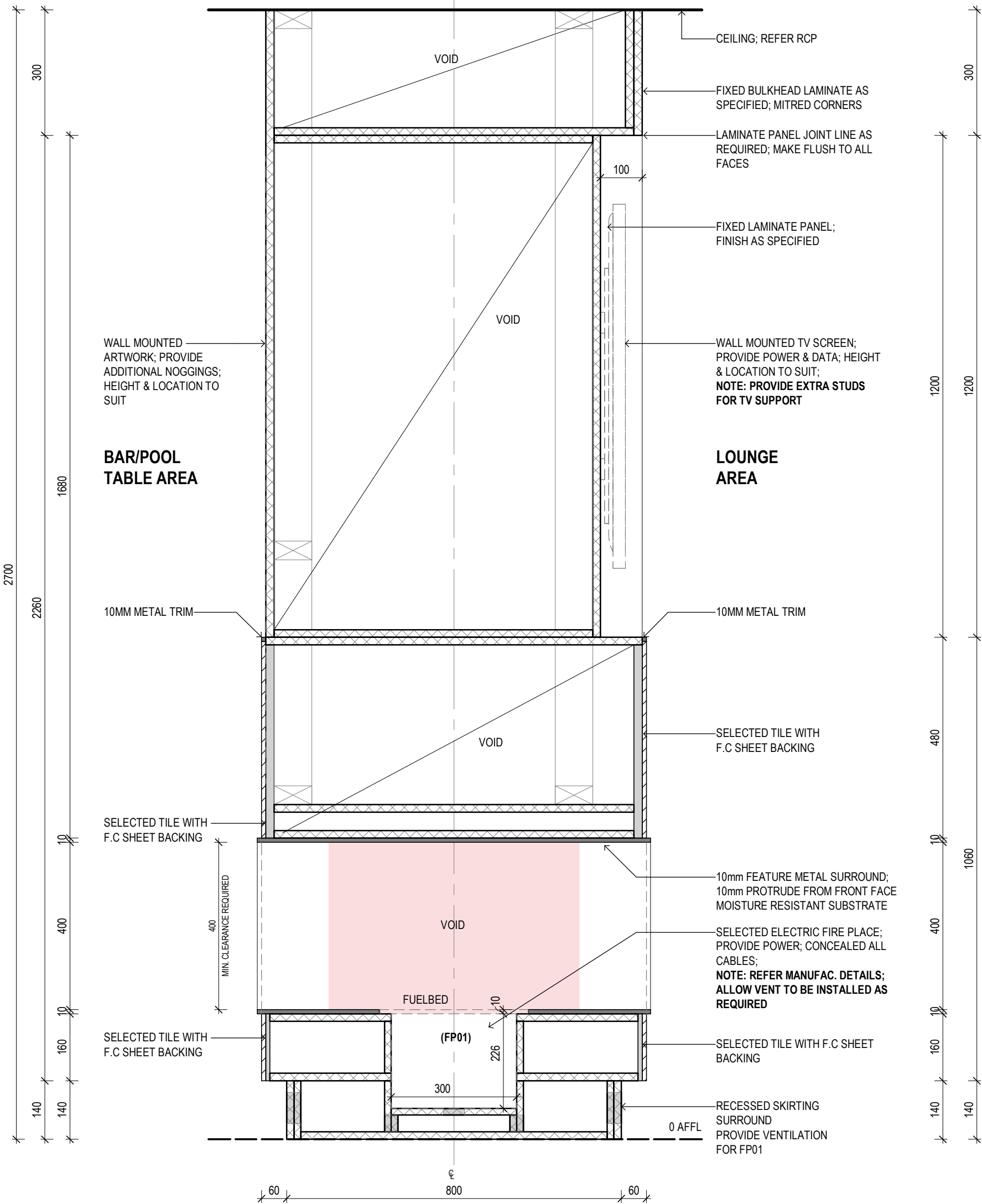
A J-04 - SPORTS BAR JOINERY SECTION A Scale 1 : 10
