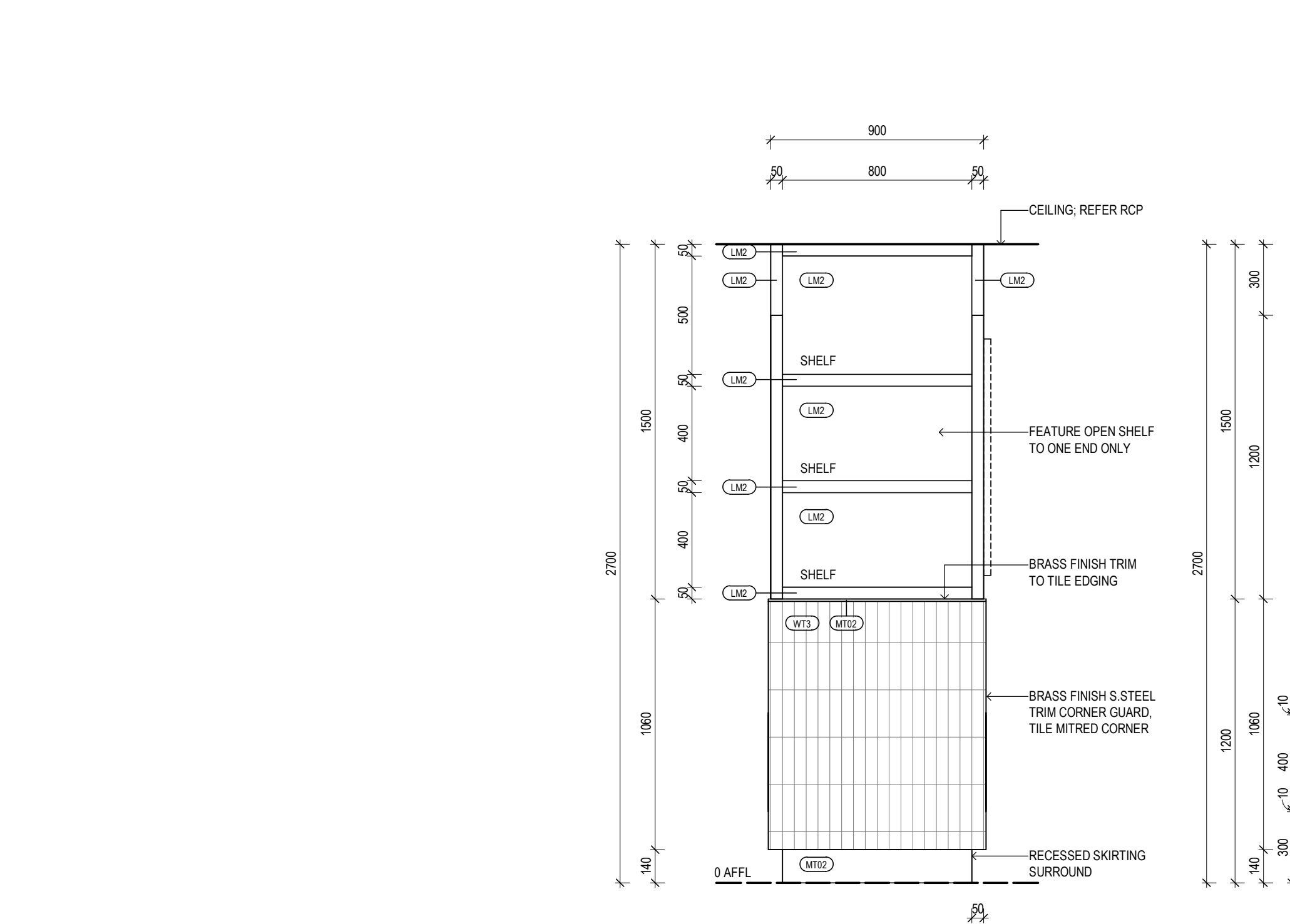
J-04 - Sports Bar Joinery ELEVATION 3 Scale 1 : 20
