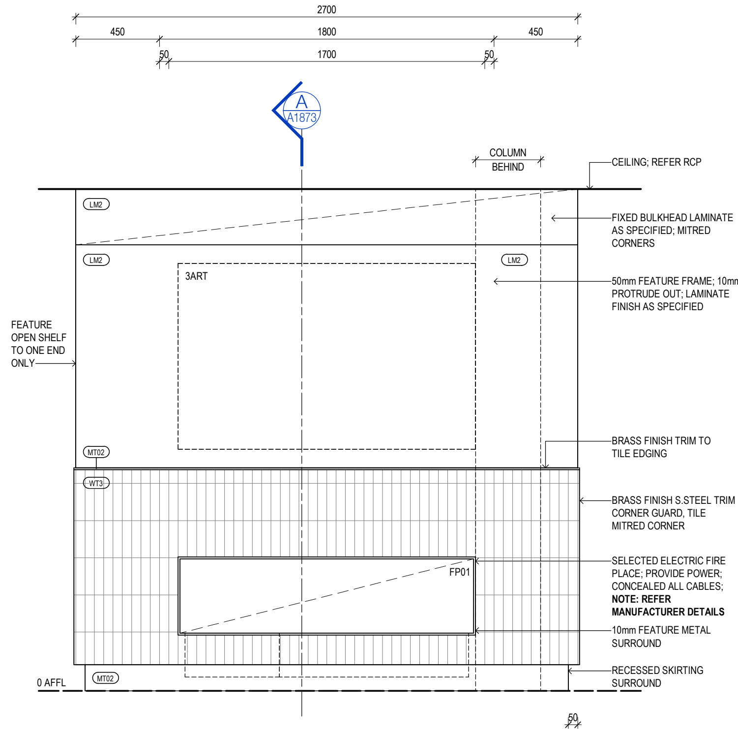
J-04 - Sports Bar Joinery - Bar/Pool Table Side ELEVATION 2 Scale 1 : 20
